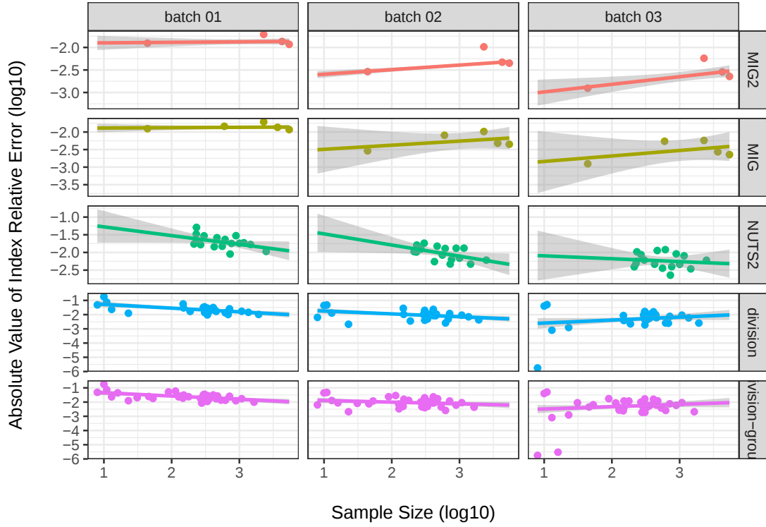
Figure 9: Absolute index error vs. sample size by breakdown and data batch.
